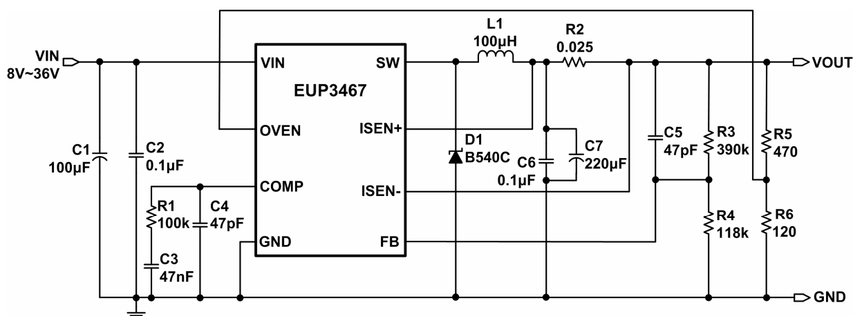
Figure 1. Application Circuit
