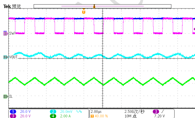
Figure 17. SW and Vout Ripple
