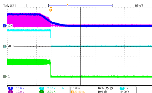
Figure 14. Power down
