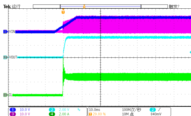
Figure 13. Power up
