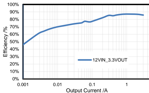
Figure 3. Efficiency vs Load Current, Vin=12V
