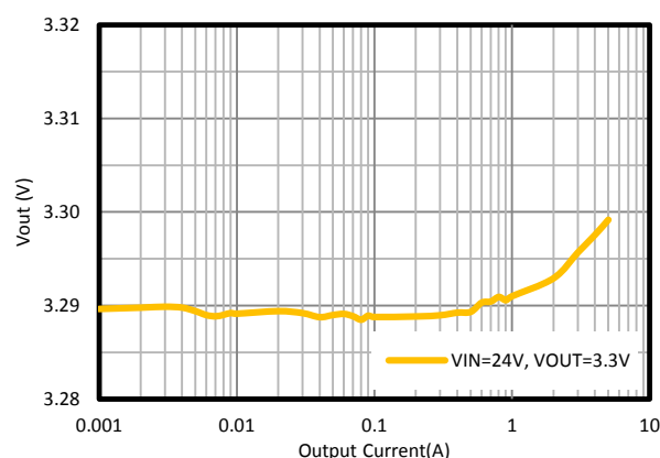
Figure 4. Load Regulation, Vin=24V
