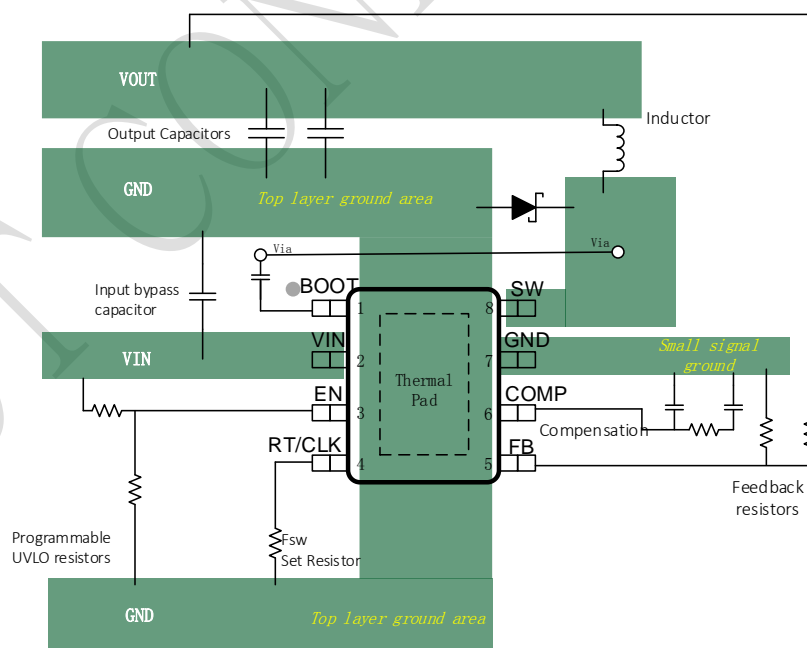
Figure 19. PCB Layout Example
