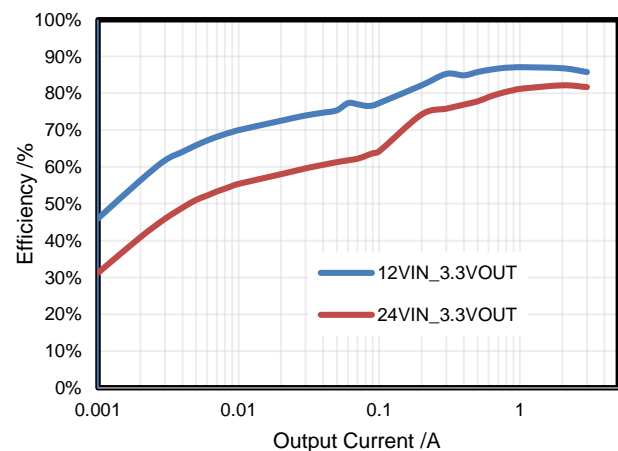
Vout=3.3V, Fsw=500KHz
