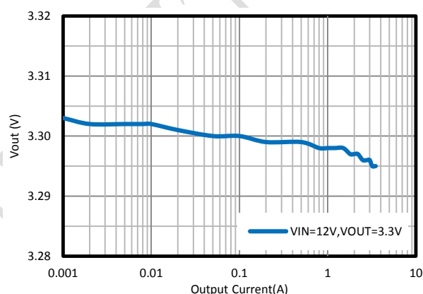
Figure 5. Load Regulation, Vin=12V
