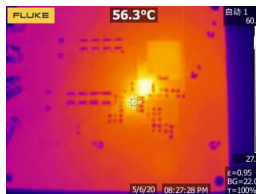
Figure 18. Thermal, 12VIN, 3.3Vout, 3A
