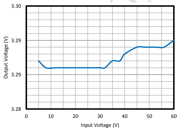
Figure 6. Line Regulation, Load=0A
