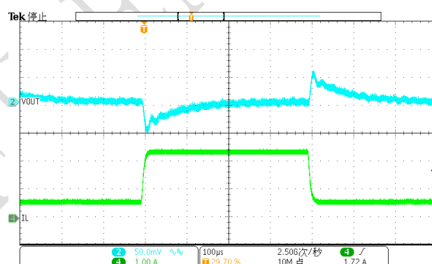
Figure 16. Load Transient (0.6A-2.4A, 1.6A/us)
