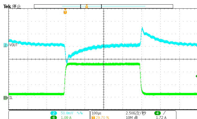
Figure 15. Load Transient (0.3A-2.7A, 1.6A/us)
