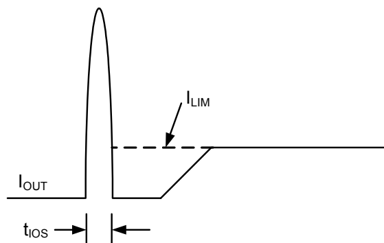
Figure 3. Response Time to Short Circuit Waveform
