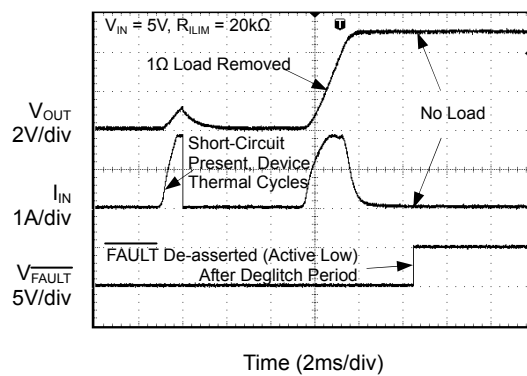
1Ω to No-Load Transient Response
