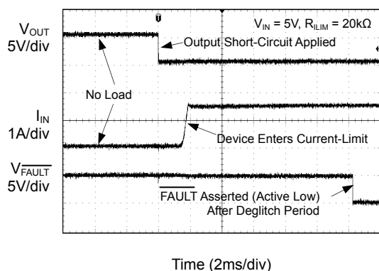
No-Load to Short-Circuit Transient Response
