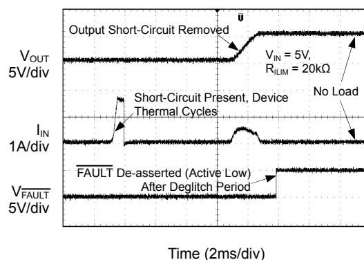
Short-Circuit to No-Load Recovery Response
