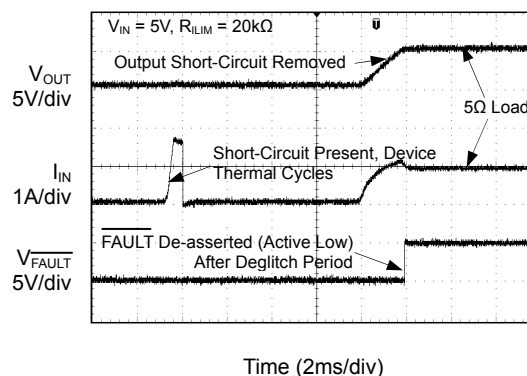
Short-Circuit to Full-Load Recovery Response
