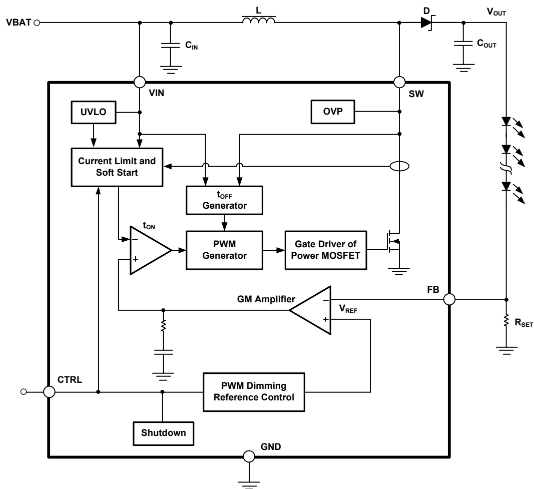
Figure 2. SGM3753 Block Diagram
