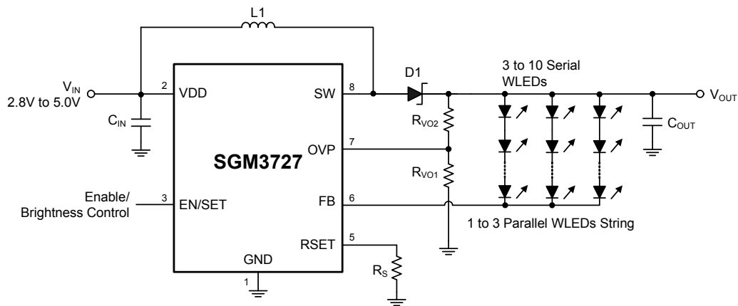
Figure 2. Application for Driving 3 × 10 WLEDs
