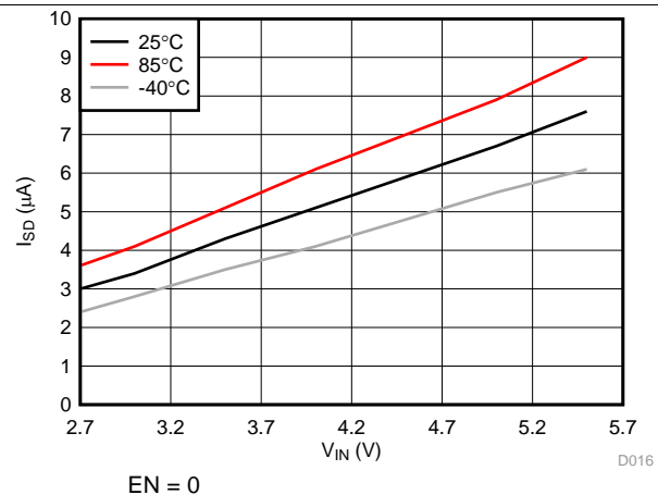
Figure 4. Shutdown Current
