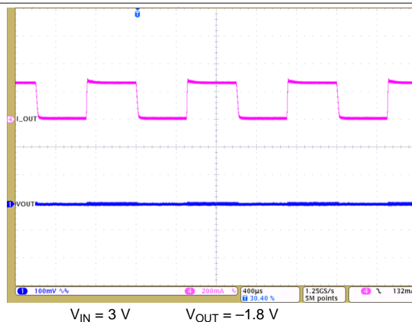
Figure 21. Load Step
