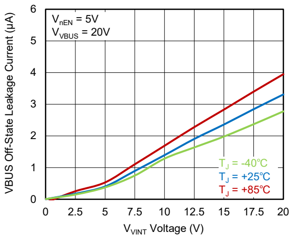
VBUS Off-State Leakage Current
