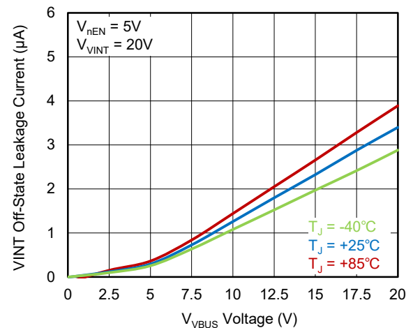
VINT Off-State Leakage Current
