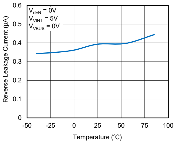
Reverse Leakage Current vs. Temperature
