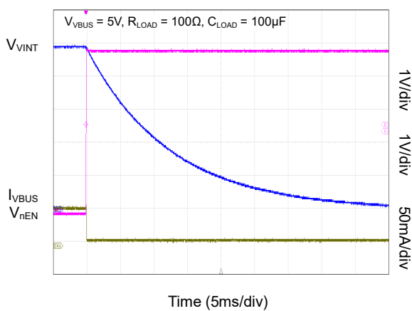
Turn-Off Time at 5V
