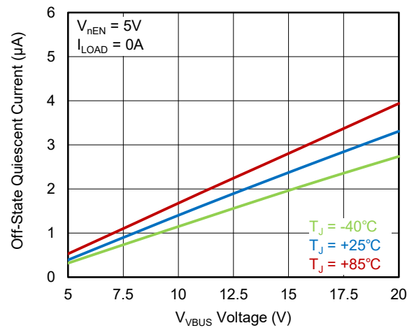
Off-State Quiescent Current vs. Input Voltage
