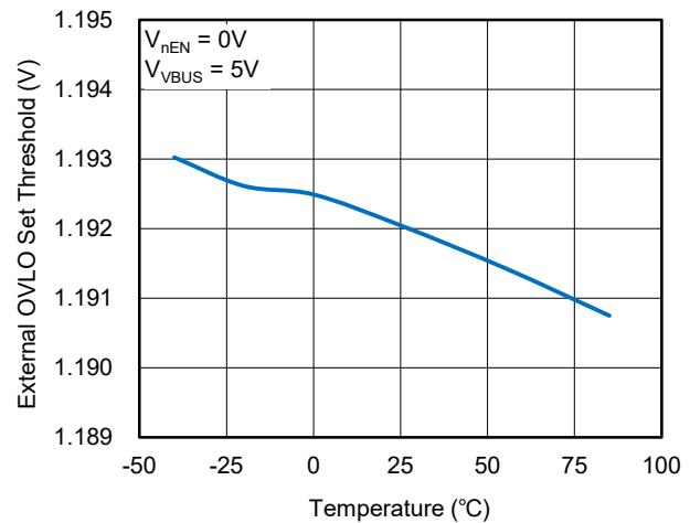
External OVLO Set Threshold vs. Temperature
