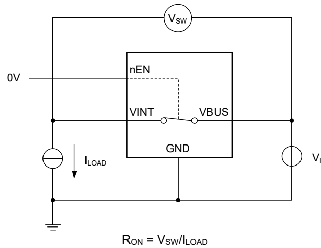
Figure 2. On-Resistance Measurement Test Circuit
