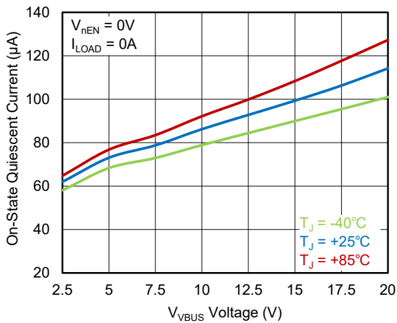
On-State Quiescent Current vs. Input Voltage
