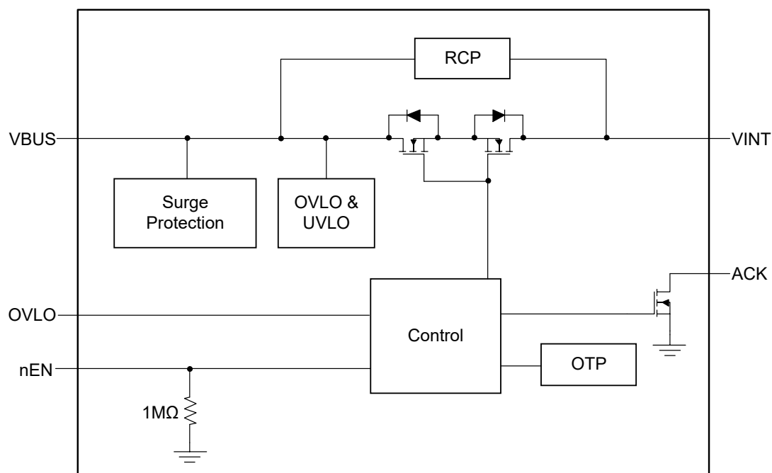
Figure 5. SGM2539 Logic Diagram
