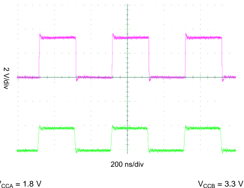
Figure 8. Level-Translation of a 2.5-MHz Signal
