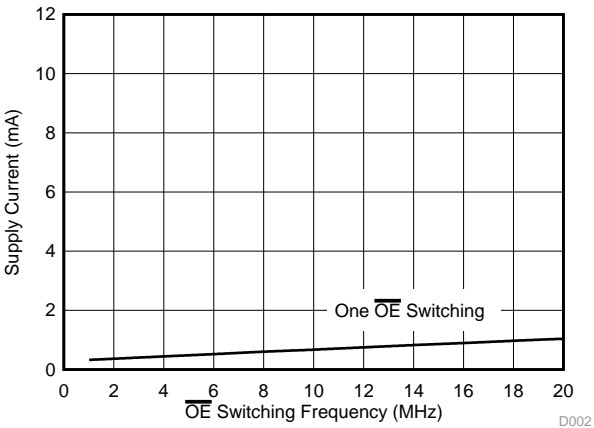
Figure 2. Typical Supply Current vs OE Switching Frequency
