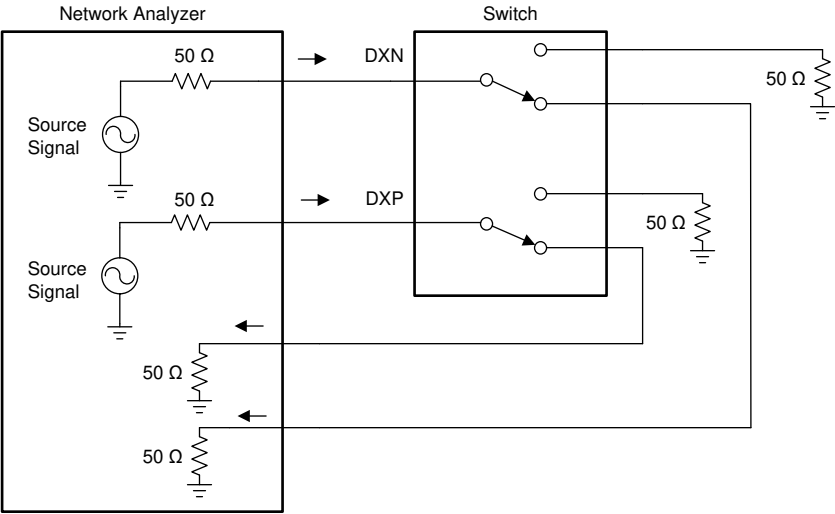
Figure 7-8. Bandwidth and Insertion Loss
