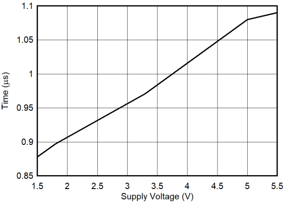
Figure 6-9. Switching Time ( t_{\text{SWITCH}} ) vs Supply Voltage
