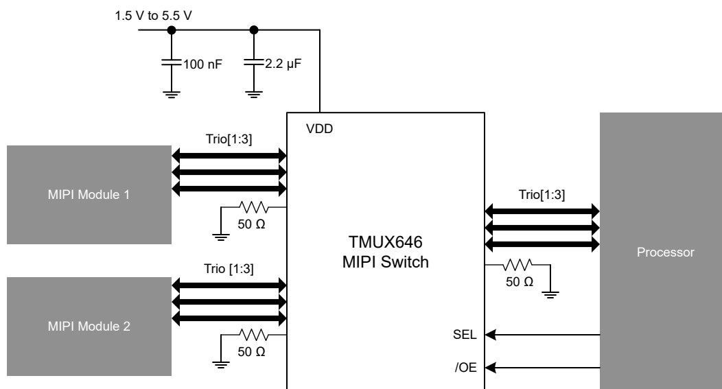
Figure 9-2. Typical C-PHY Application
