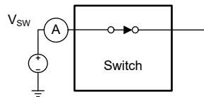
Figure 7-3. On Leakage
