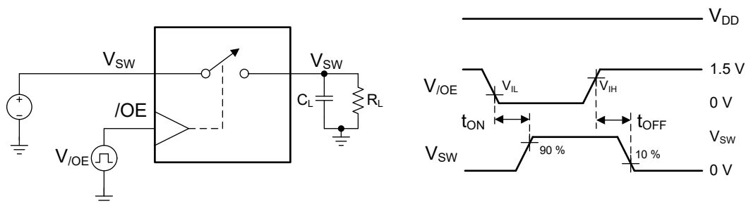
Figure 7-5. t_{\text{ON}} and t_{\text{OFF}} Timing for \overline{\text{OE}}
