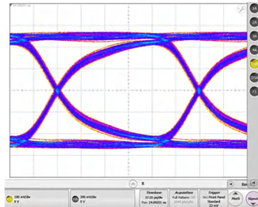
Figure 9-6. 4.5 Gbps with TMUX646 (500-mV pp )
