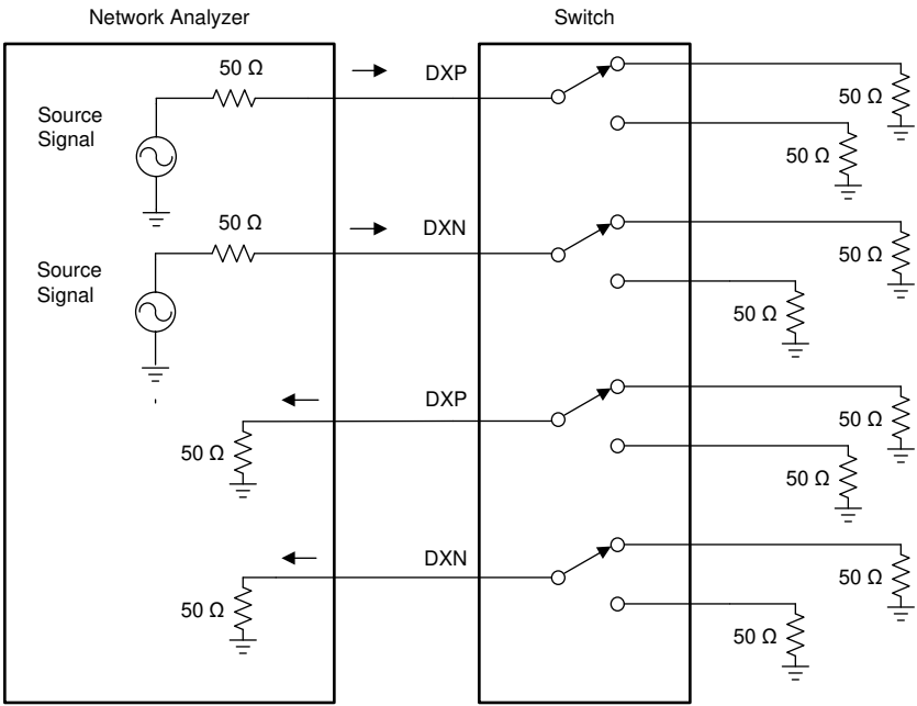
Figure 7-7. Crosstalk
