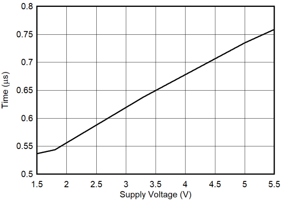
Figure 6-12. t_{\text{OFF\_VDD}} vs Supply Voltage
