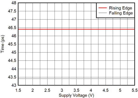
Figure 6-10. Propagation Delay ( t_{\text{PD}} ) vs Supply Voltage
