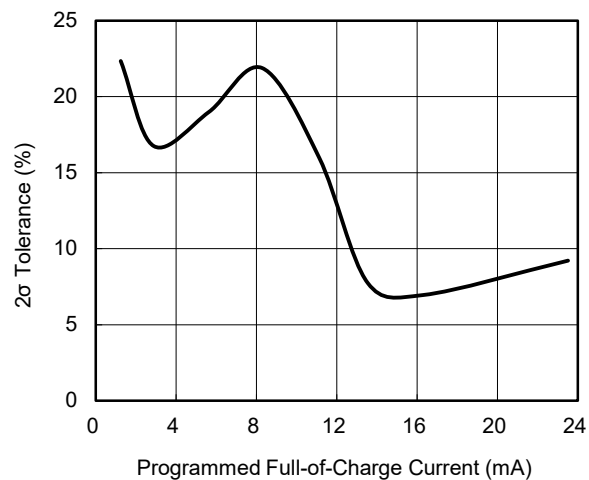
Full-of-Charge Current Programming 2 \sigma Tolerance Guide
