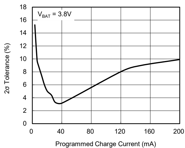
Charge Current Programming 2 \sigma Tolerance Guide
