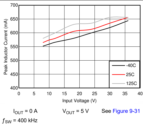
Figure 7-6. I_{PEAK-MIN}
