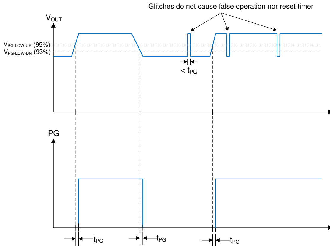
Figure 8-2. Power-Good-Timing Behavior
