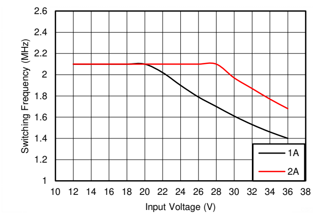
Figure 8-13. Switching Frequency versus Input Voltage V_{OUT} = 3.3\text{ V}
