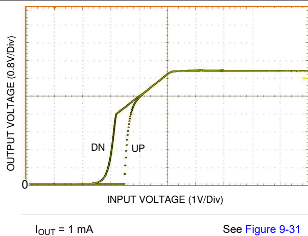
Figure 7-5. UVLO Thresholds
