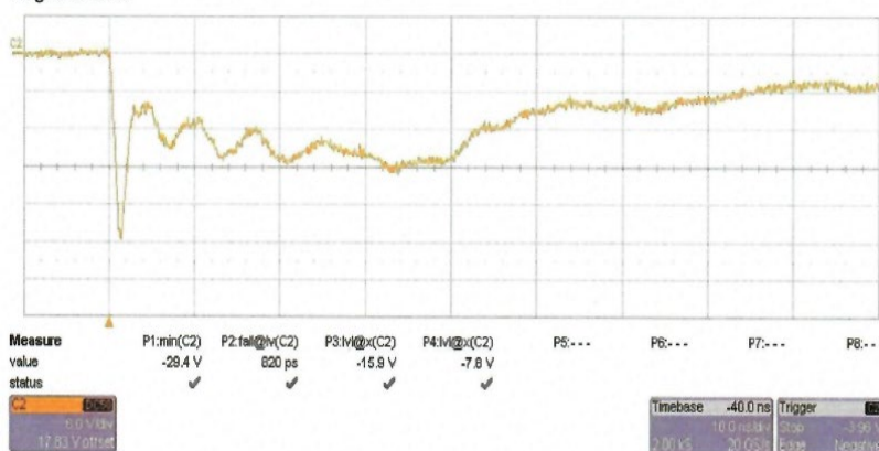
Figure 2. Typical Pulses ESD -8kV Contact per IEC 61000-4-2
