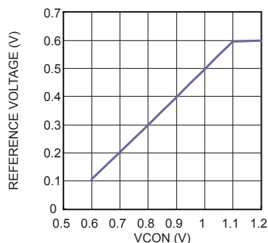
Figure 5: Reference Voltage change with VCON
