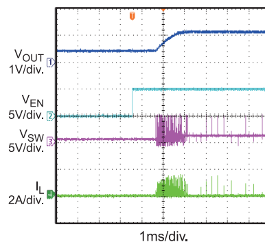
V_{OUT} Prebias Start Up
